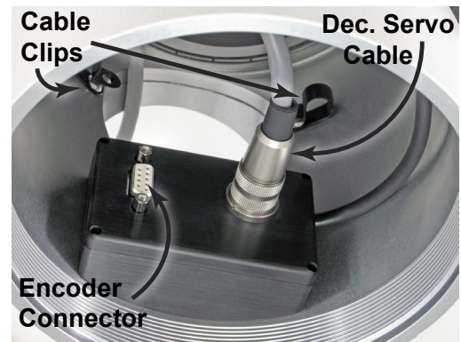
Dec. Counterweight Adapter Removed
